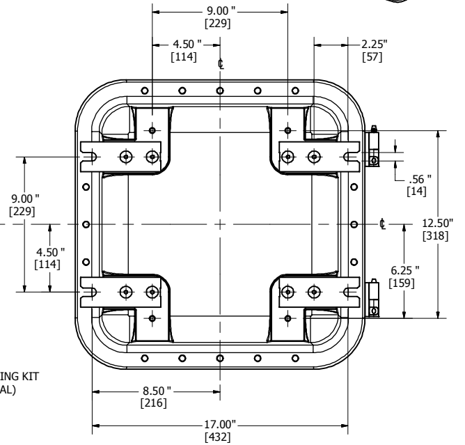
MOUNTING FEET
